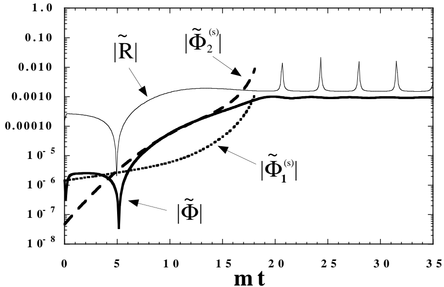
FIG. 3: The evolution of the metric perturbation \tilde{\Phi} \equiv k^{3/2}\Phi and the curvature perturbation \tilde{\mathcal{R}} \equiv k^{3/2}\mathcal{R} with same parameters as in Fig. 2. The amplification of field perturbations leads to the nonadiabatic growth of \Phi and \mathcal{R} . We also plot \tilde{\Phi}_1^{(s)} \equiv k^{3/2}\Phi_1^{(s)} and \tilde{\Phi}_2^{(s)} \equiv k^{3/2}\Phi_2^{(s)} , where \Phi_1^{(s)} and \Phi_2^{(s)} denote the first and the second terms in Eq. (4.34), respectively. \Phi is mainly sourced by the \Phi_2^{(s)} term, after \Phi_2^{(s)} catches up \Phi_1^{(s)} . The evolution of \Phi_1^{(s)} and \Phi_2^{(s)} after inflation is not shown.
